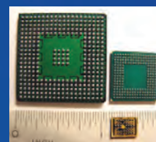
BGA
